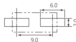
Land Pattern
