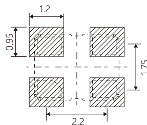
Land Pattern
