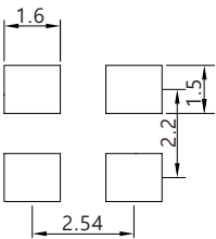
Land Pattern
