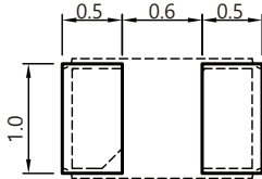
Land Pattern
