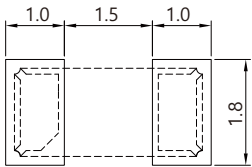
Land Pattern
