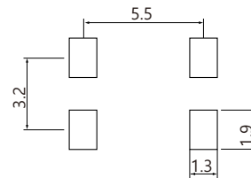
Land Pattern
