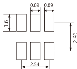
Land Pattern
