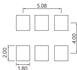
Land Pattern
