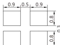
Land Pattern
