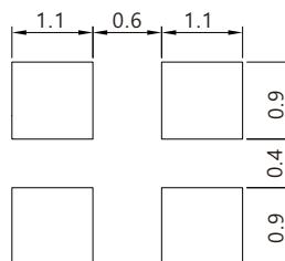
Land Pattern
