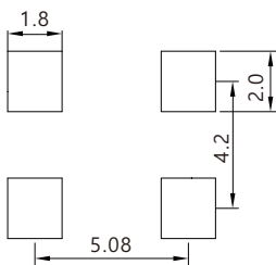
Land Pattern
