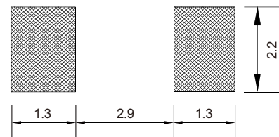
Land Pattern
