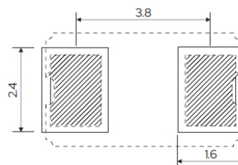
Land Pattern
